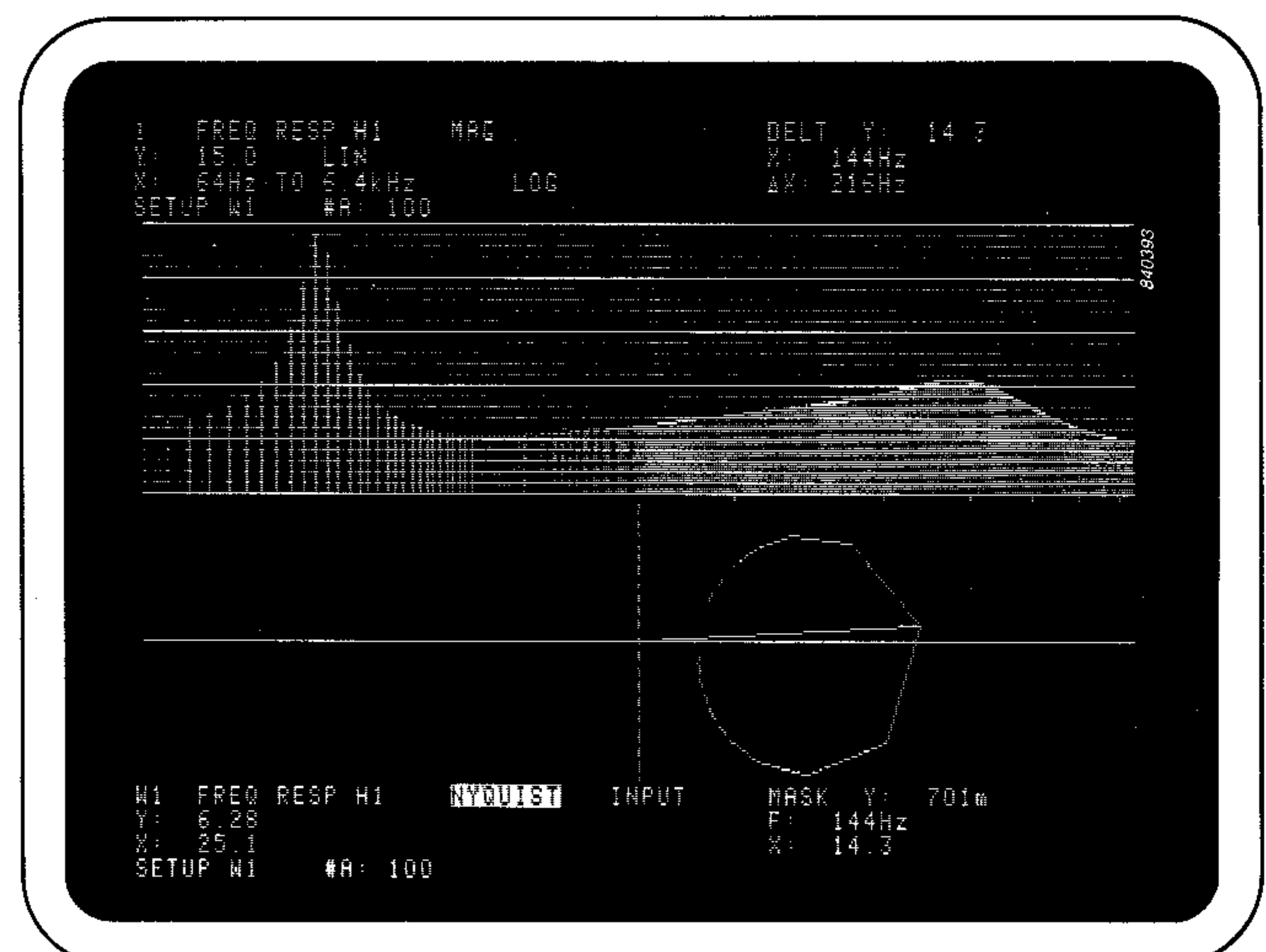
Fig. 24. Linear magnitude and Nyquist plot of loudspeaker impedance. A large (800 line) Fourier Transform is essential for obtaining an adequate resolution for simultaneous measurement of both resonance peaks. The "MASK" cursor used with the Nyquist plot helps eliminate the confusion often associated with such plots. The trace represents the frequency range indicated by the delta cursor in the upper display. Each resonance peak in the impedance plot will correspond to a full circle in the Nyquist plot
