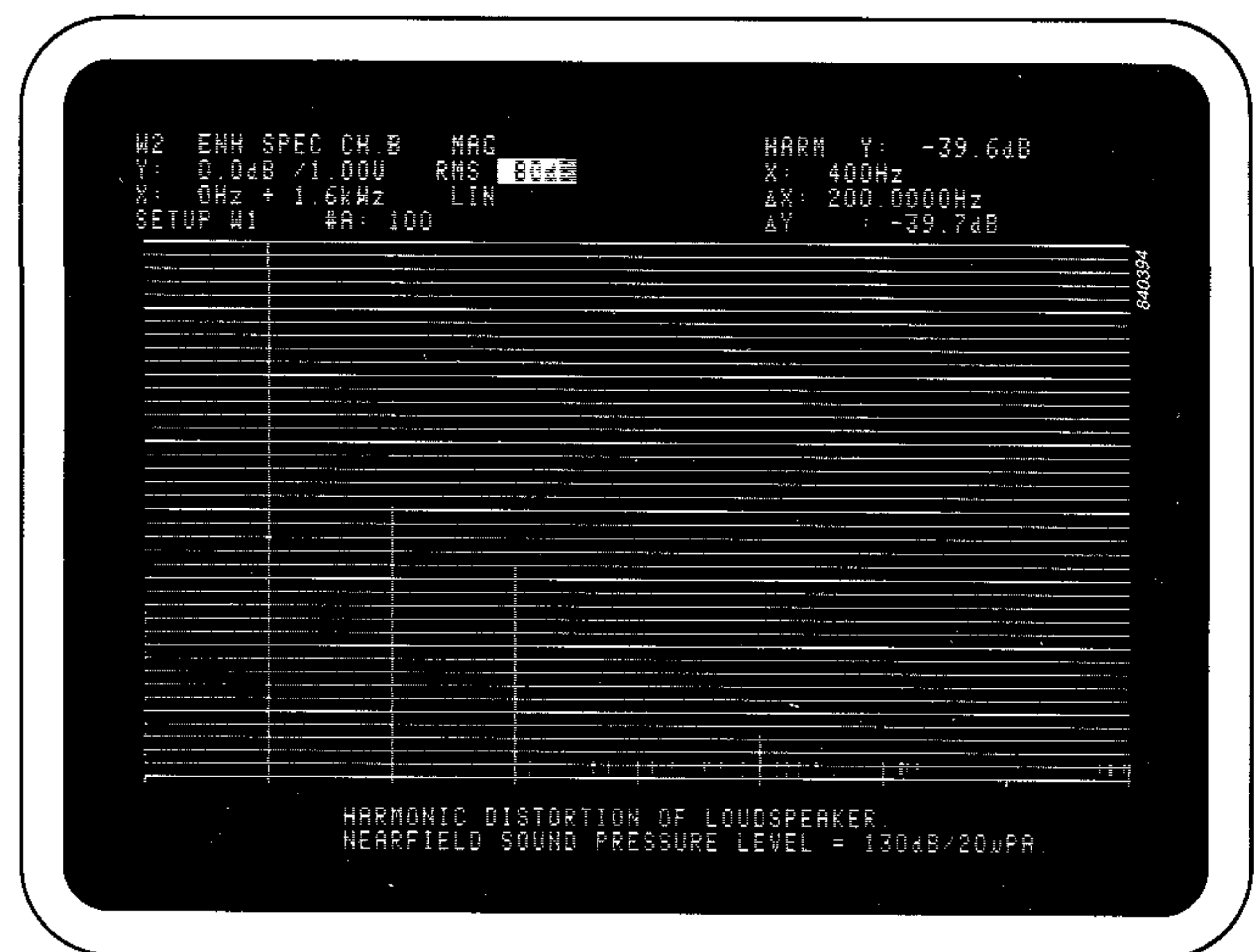
Fig. 25. Near-field measurement of harmonic distortion measured near the low frequency resonance of the loudspeaker. However, the sound pressure level should normally refer to the level at 1m distance from the loudspeaker. The cursor indicates a second harmonic distortion of -39,7\text{dB} relative to the fundamental
