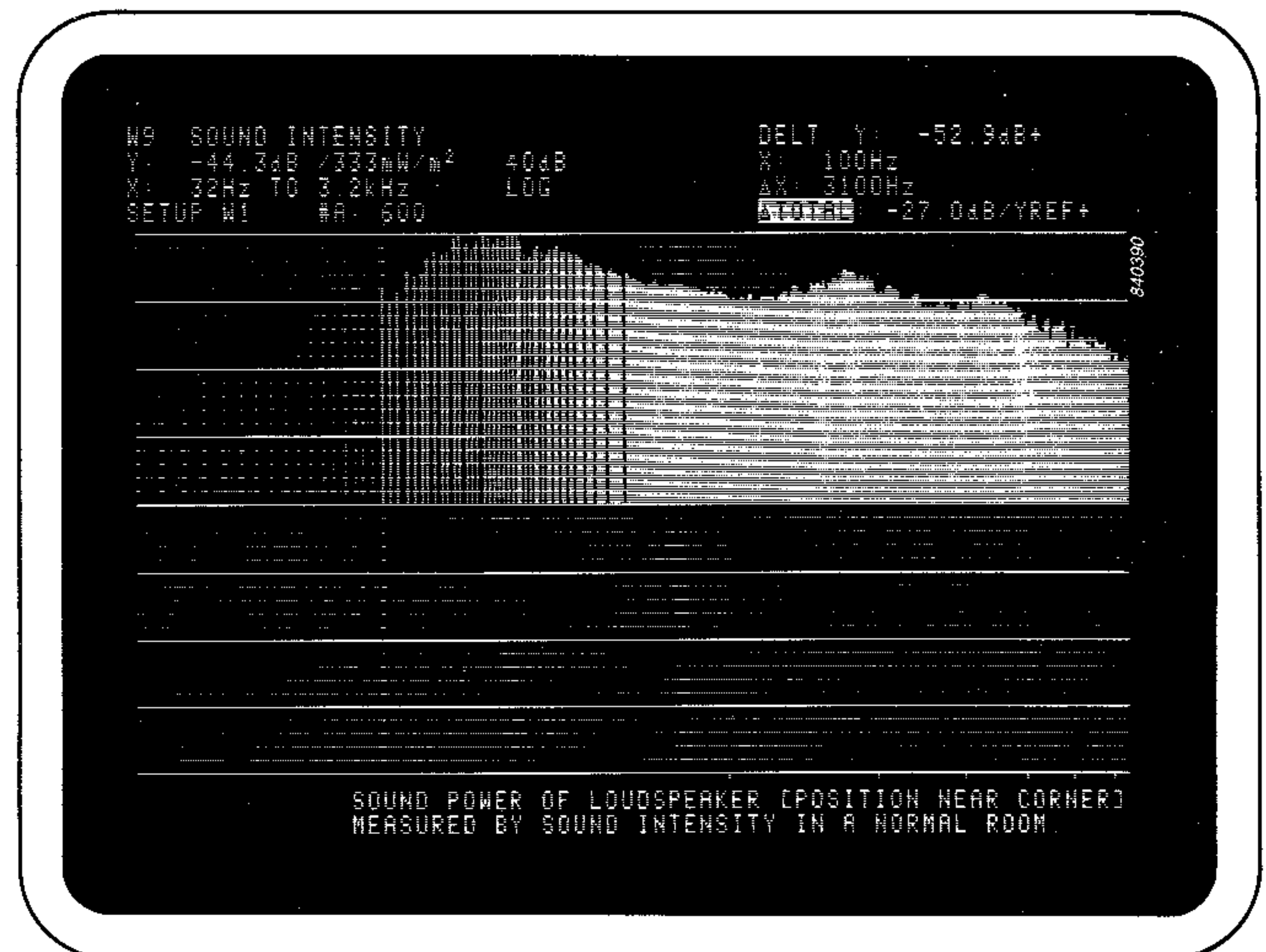
Fig. 23. Sound power measured as in Fig. 22, but with the loudspeaker positioned near a corner where the acoustical impedance better matches the radiation impedance of the speaker. This results in a higher acoustical output in the low frequency range. Due to the absorbing surfaces near the corner, the response in the upper part of the displayed range is lower than the response shown in Fig. 22
